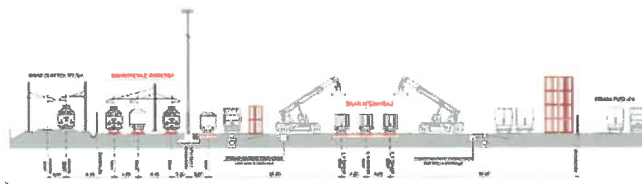
Actual typical section of the intermodal terminal
